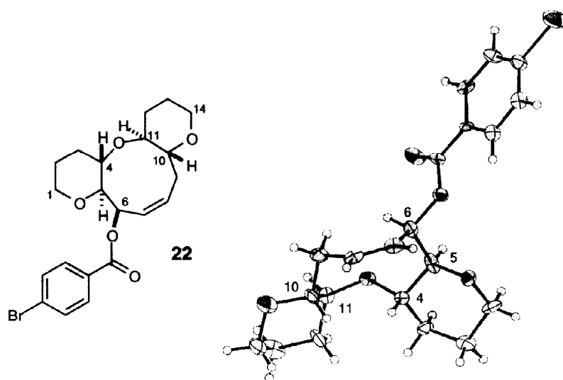
Figure 3. ORTEP drawing of p -bromobenzoate 22
