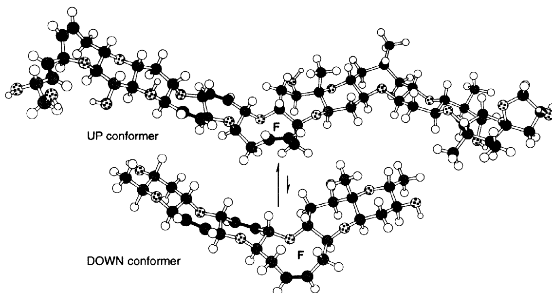
Figure 2. Possible Conformers of Ciguatoxin
