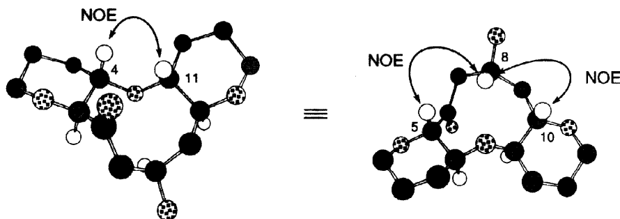
Figure 4. Energy-minimized structure (Macromodel, MM2* force field) and NOE data for compound 2
