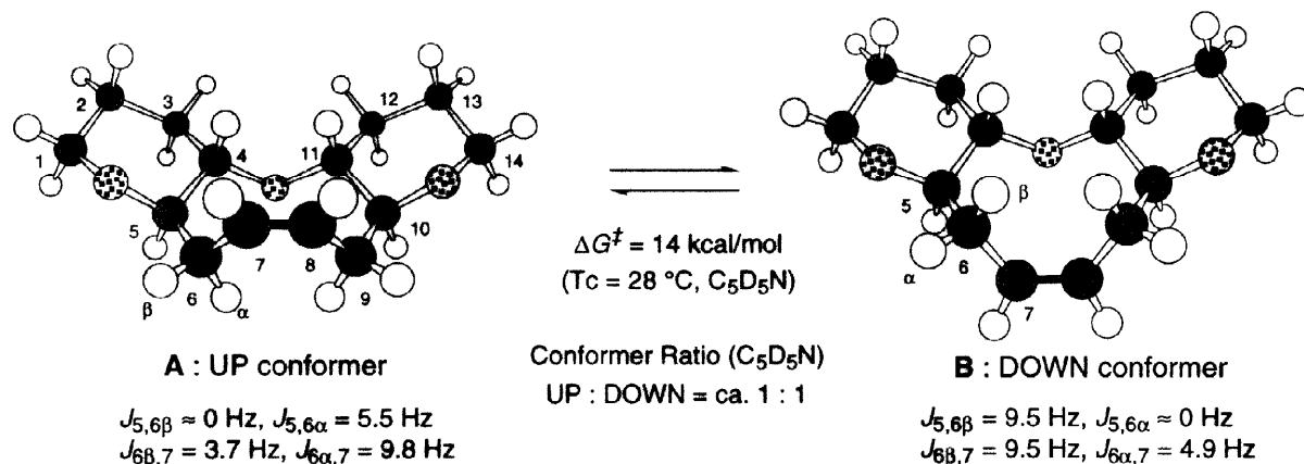
Figure 5. Conformational alteration of 6-9-6 tricyclic model compound 1
