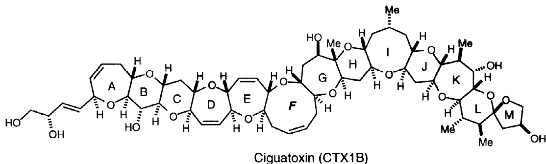
Figure 1. Absolute Structure of Ciguatoxin (CTX1B)
